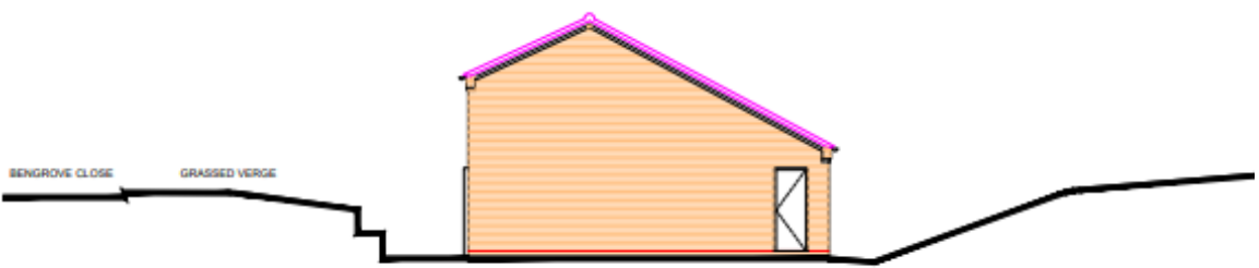
SECTION ON NORTH WEST ELEVATION: AS EXISTING
