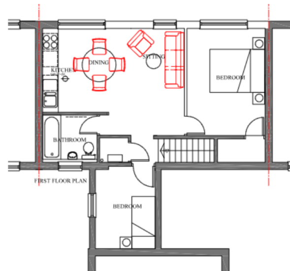
Proposed Floor Plans
