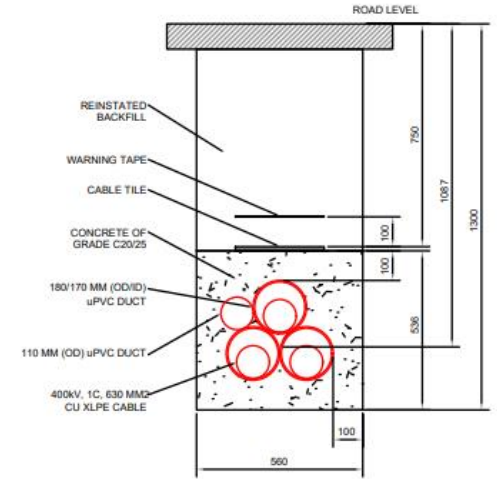
SECTION C-C TYPICAL TRENCH IN ACCESS ROAD
