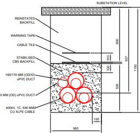
SECTION A-A TYPICAL TRENCH IN SUBSTATION
